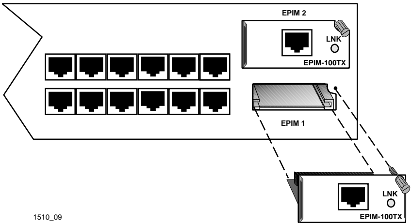
Figure 4-6 Installing an EPIM
